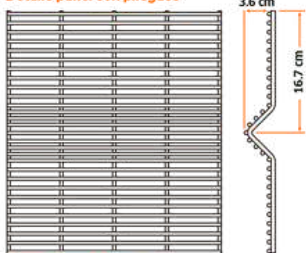
Detalle panel plano
